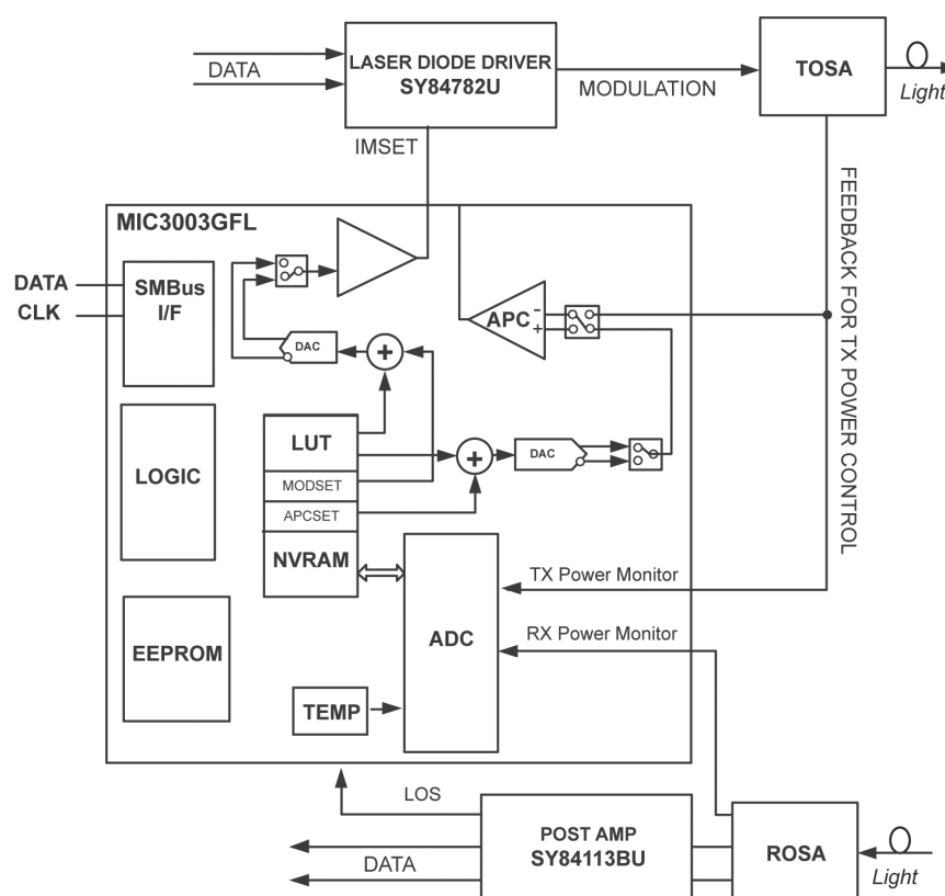
SFP/SFF Optical Module
