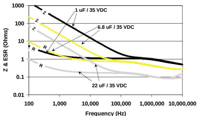
FIGURE 9a ESR & Impedance (Z) vs Frequency
