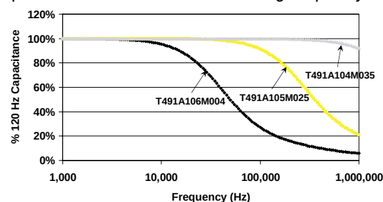
FIGURE 1 Typical Effect of Frequency upon Capacitance
